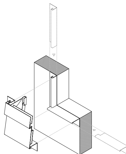
BASE ASSEMBLY PERSPECTIVE
